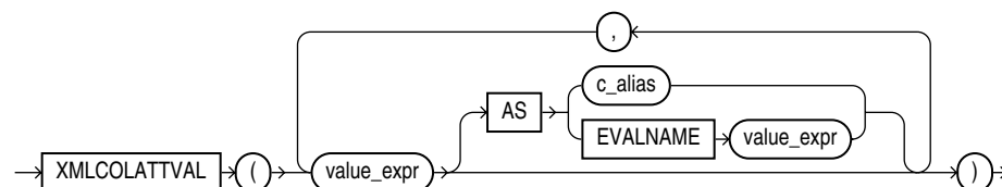
Figure 18–11 XMLCOLATTVAL Syntax
