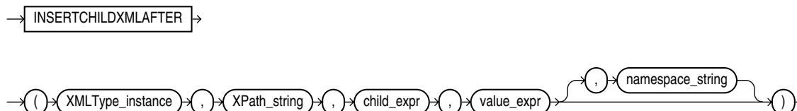
Figure 4–6 INSERTCHILDXMLAFTER Syntax
