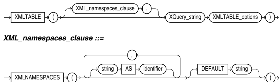
Figure 5-2 XMLTABLE Syntax
