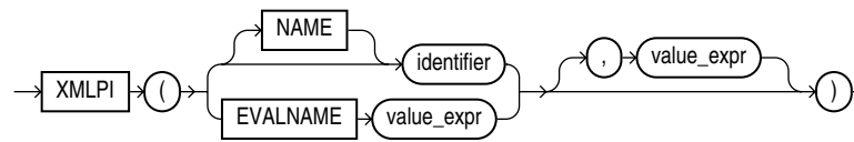
Figure 18–6 XMLPI Syntax
