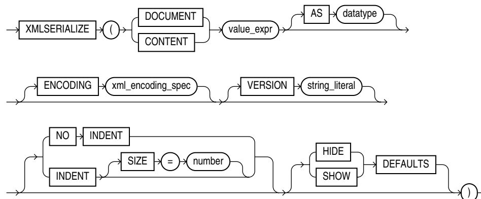
Figure 18-8 XMLSerialize Syntax
