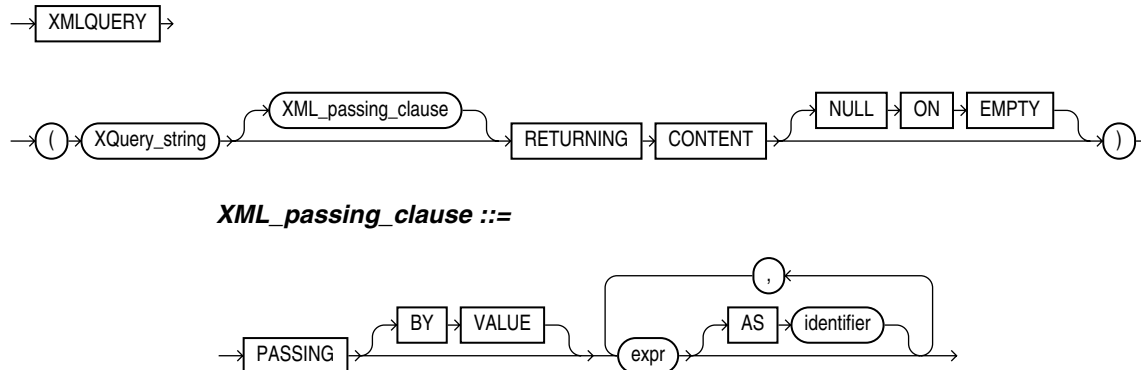
Figure 5–1 XMLQUERY Syntax
