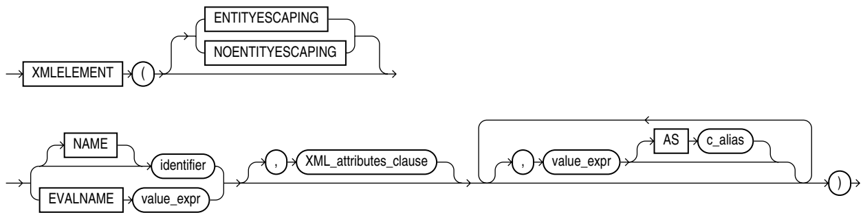
Figure 18–1 XMLelement Syntax
