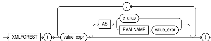
Figure 18–3 XMLFOREST Syntax
