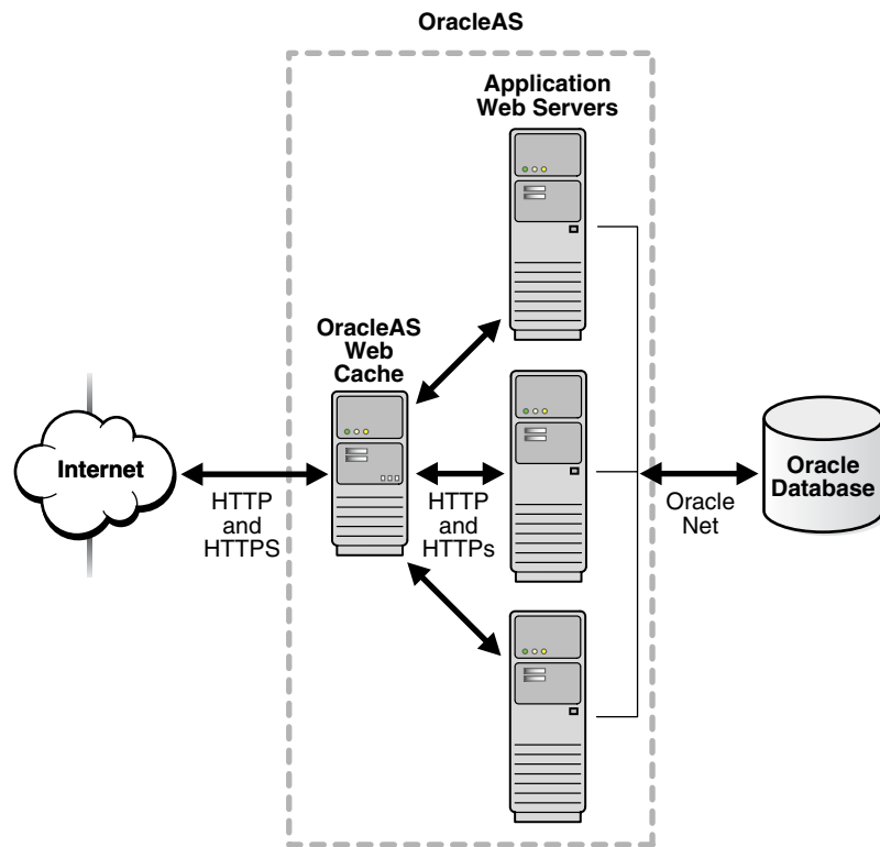
Figure 11–1 Middle-Tier Caching
