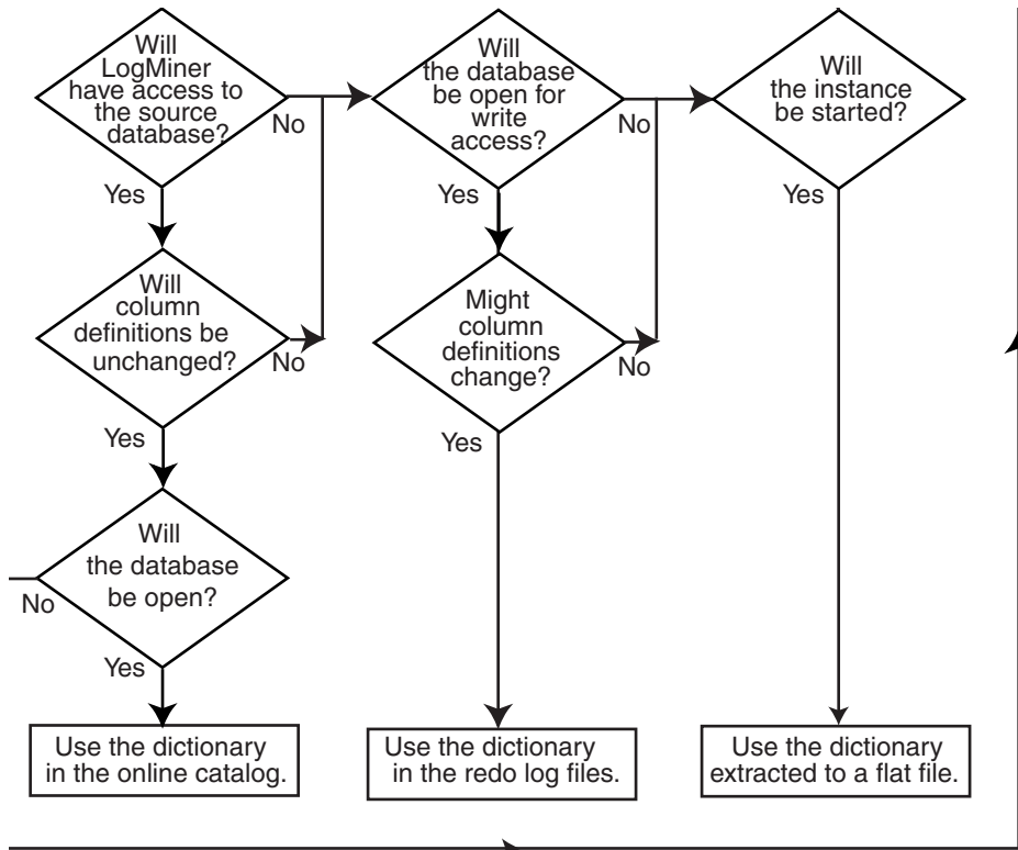
Figure 19–2 Decision Tree for Choosing a LogMiner Dictionary
