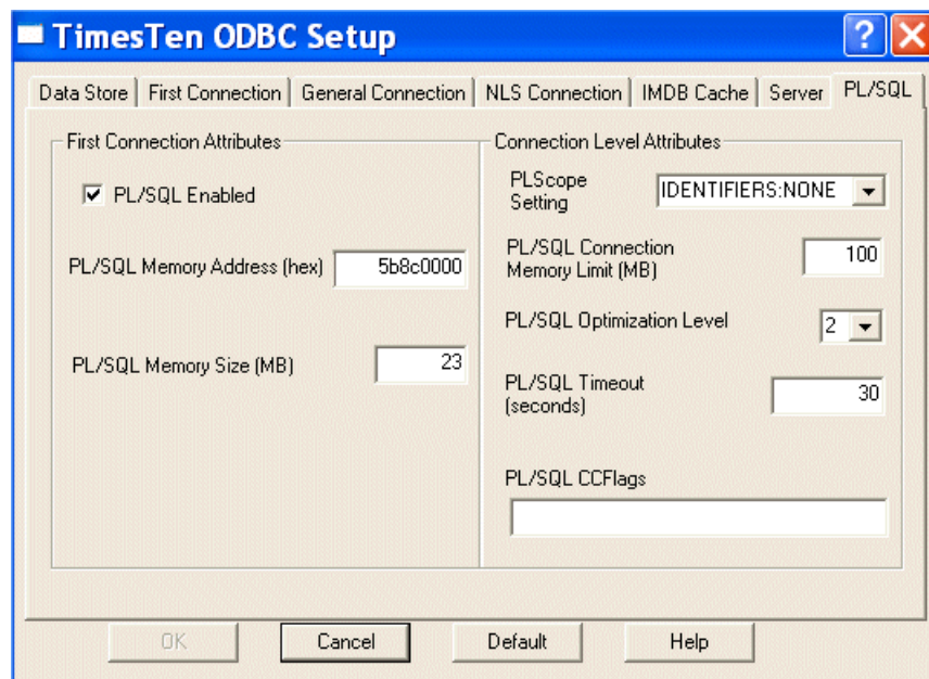
Figure 1–8 PL/SQL Attributes
