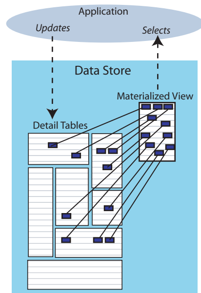
Figure 7-1 Materialized view
