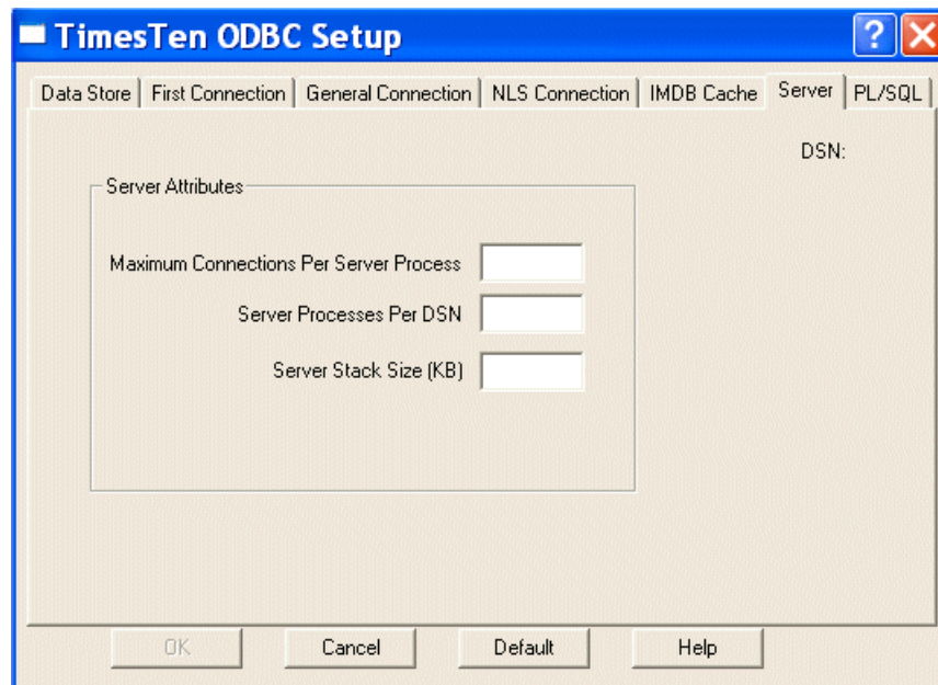
Figure 1–7 Server Attributes
