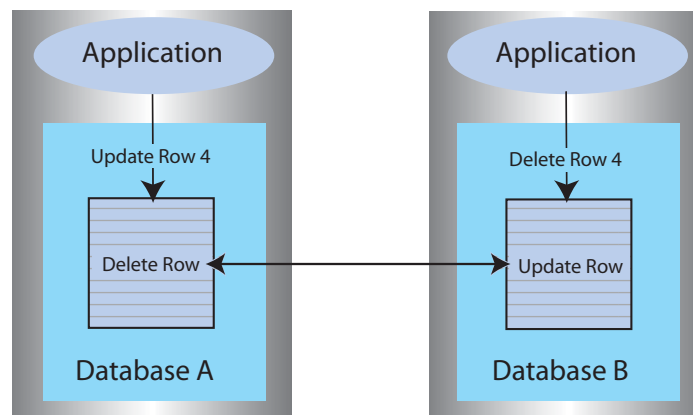
Figure 15-2 Delete/update conflict
